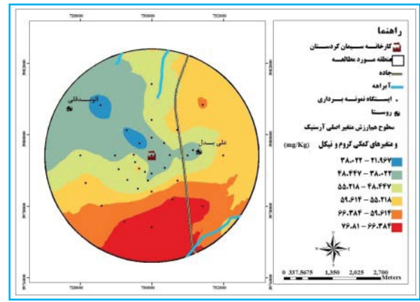
(As)
