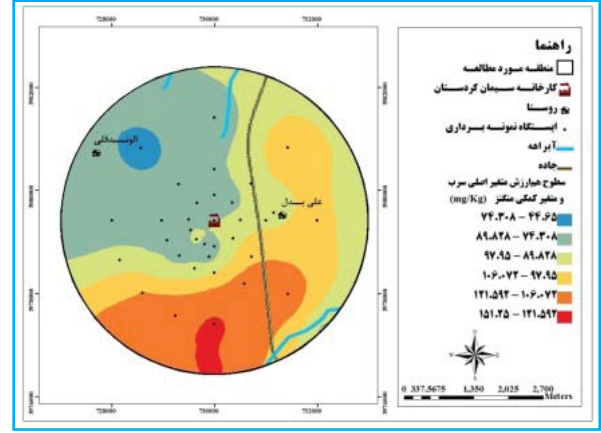
(Pb)
