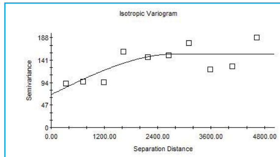
(As)
