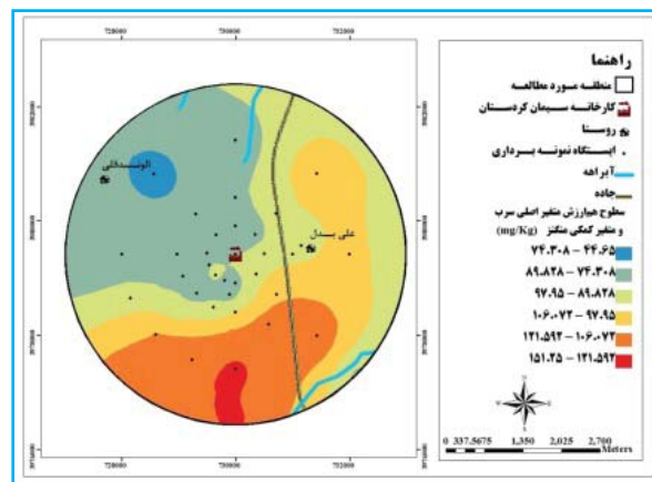
(Pb)
