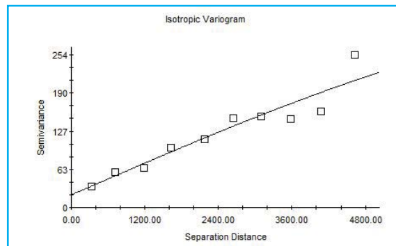
(As)
