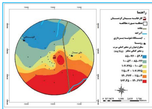
(Pb)
