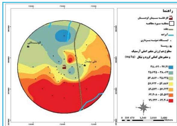
(As)
