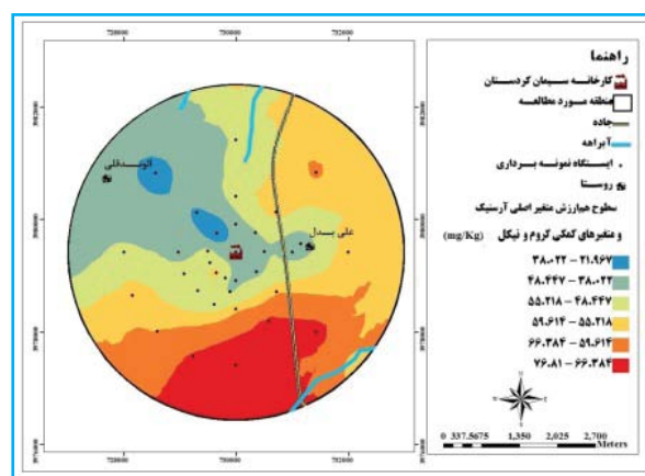
(As)
